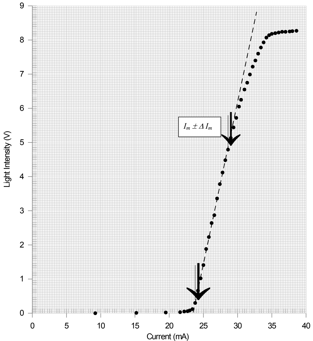
Fig. A-1 Graph of light intensity I versus current I
