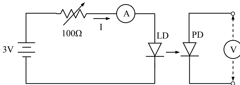
Fig. 5 Equivalent circuit for the connection of the laser diode.
