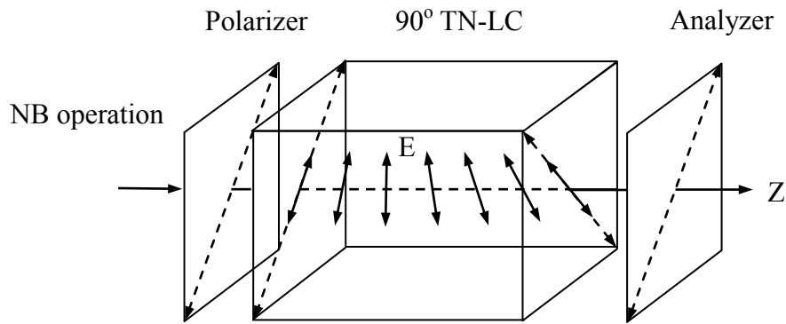
Fig. 9 NB mode operation of a 90° TN cell
