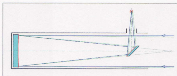
4. Galaxy.
