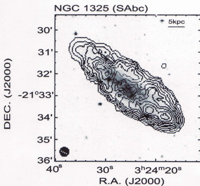
4. Galaxy.
